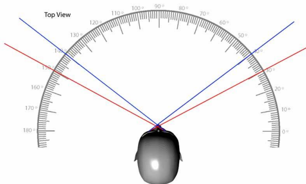
Human Stereoscopic Field of View
